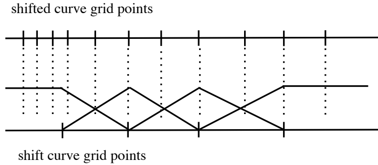
Figure 32: 1-d shift curve (bottom) applied to a more granular underlying curve (top).
